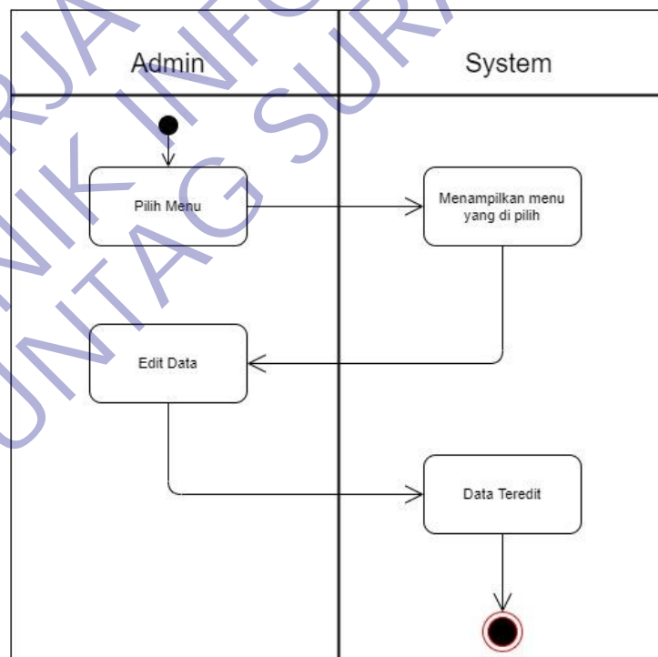
Gambar 12 Activity Diagram Edit Data. Source: Dokumentasi Pribadi
