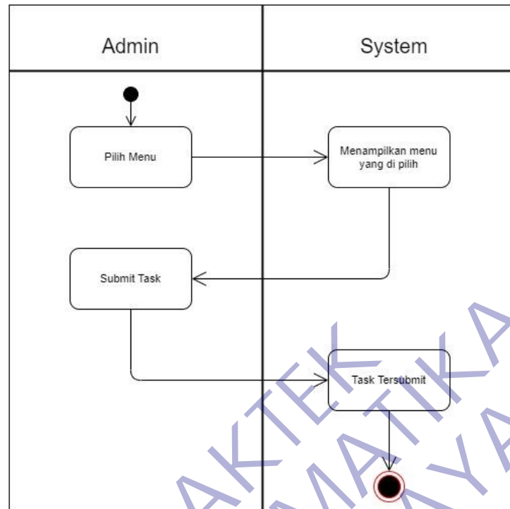
Gambar 13 Activity Diagram Submit Task. Source: Dokumentasi Pribadi
