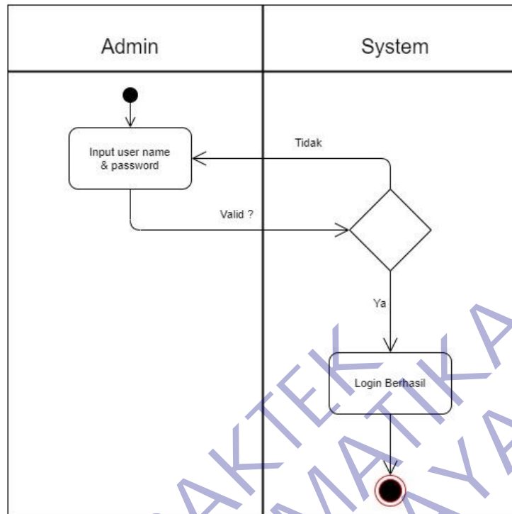
Gambar 9 Activity Diagram Login. Source: Dokumentasi Pribadi
